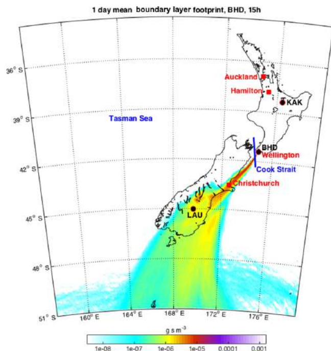
Figure 2. Air history map for 10000 particles released at BHD during 15:00–16:00LT on 19 May 2012 using the NAME III model. The particle back trajectories show a southerly event locally at the station, though not a baseline event as the air crosses parts of South Island. Also shown are the locations of LAU and Kākaramea/Rainbow Mountain (KAK) stations.
